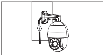
Step 9-Cable Connection
